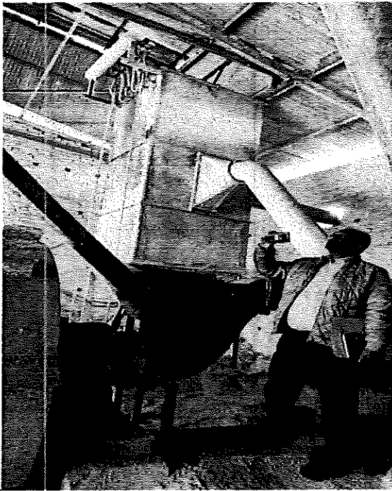
Photo 30: Photograph of Bag Filter With Ball Mill
