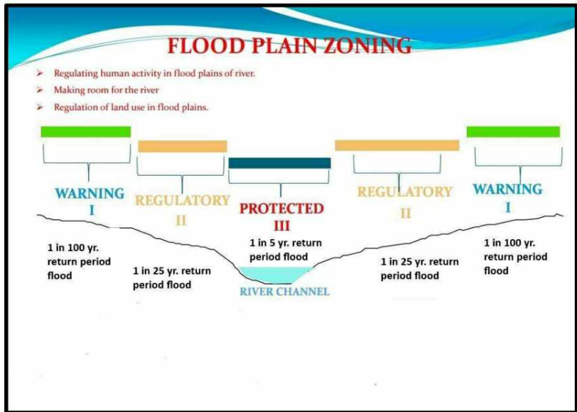
Figure 6- Flood Plain Zoning
