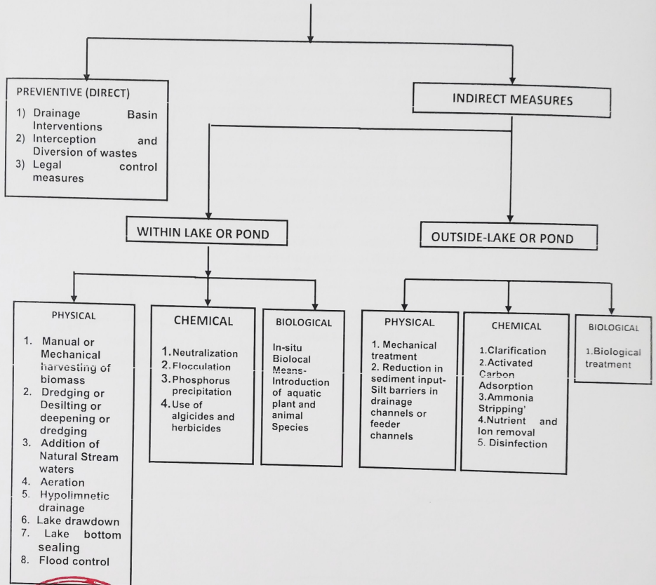
Figure 1. A Model Lake or Pond Restoration Technique
