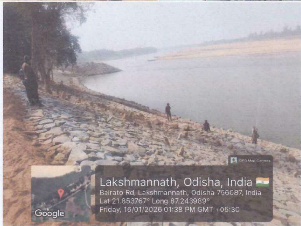
Construction of Spur along with launching & packing in left bank of river Subarnarekha near village Gobarghata
