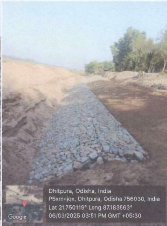
Bank protection by launching & Packing in right Bank of river Subarnarekha near village Dhitpura
