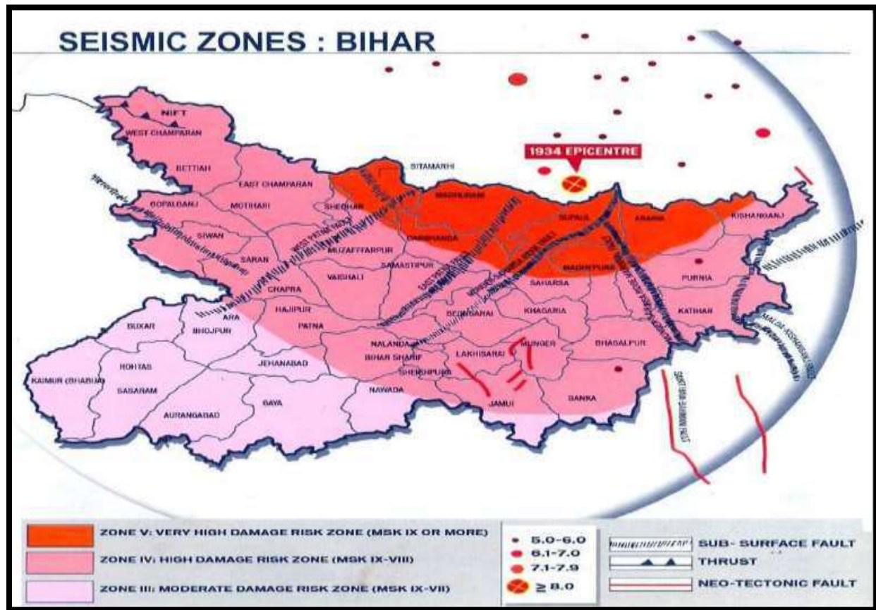
Figure 2.7: Earthquake Hazard Map of Bihar
