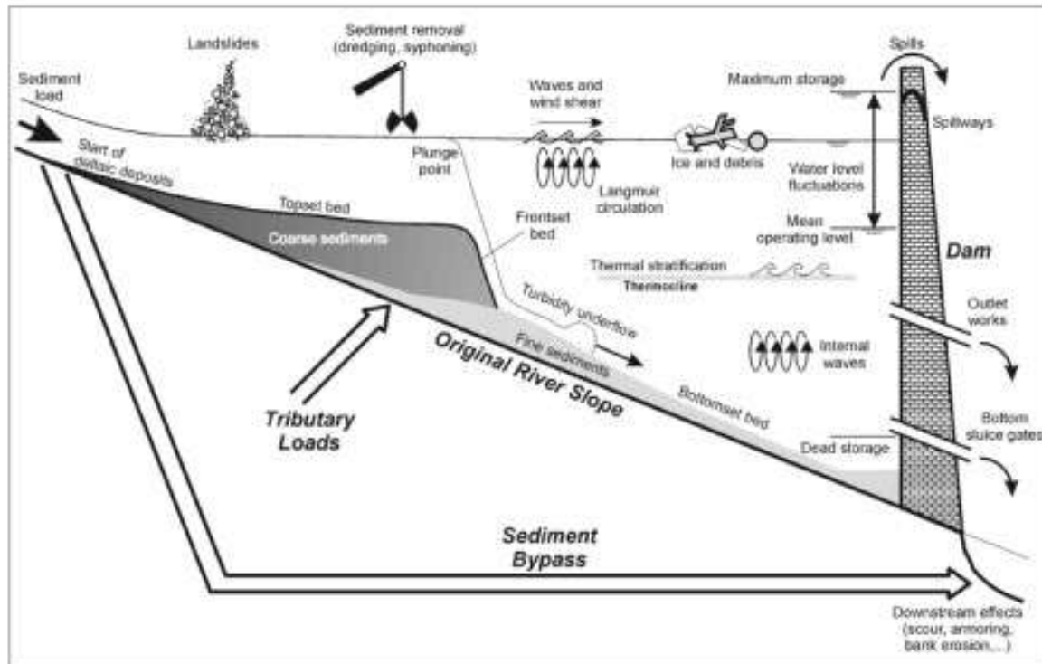
Fig 2 Sedimentation Pattern in Reservoir (USBR,2006)
