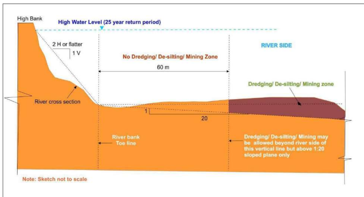
Figure 2: Typical Dredging / De-silting / Mining Restrictions for protecting natural river banks
