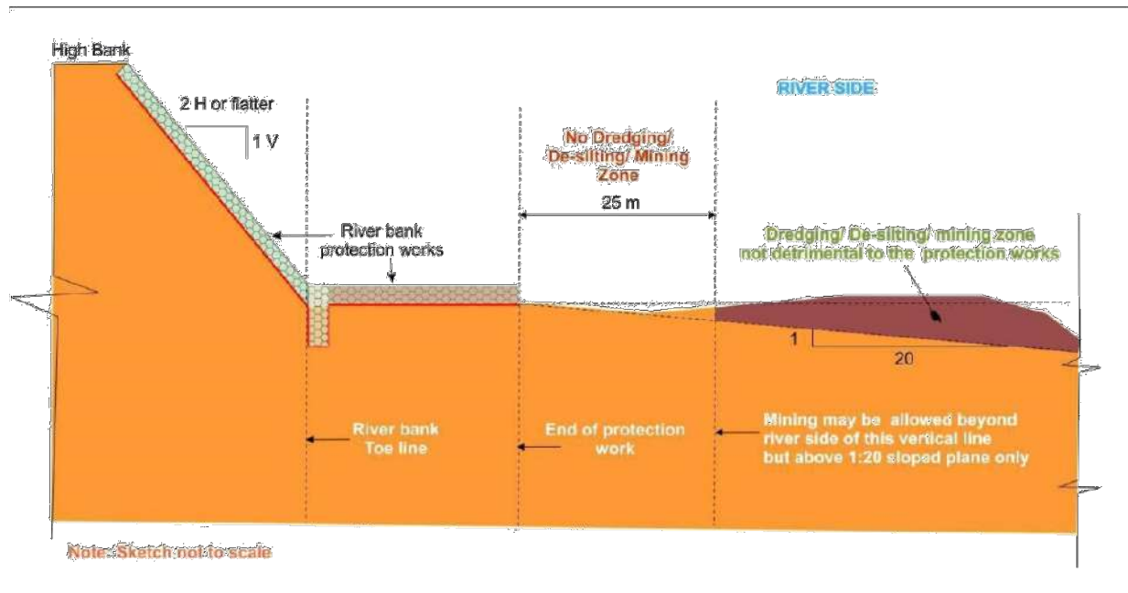
Figure 1: Typical Dredging / De-silting / Mining Restrictions for protecting river bank with bank protection works
