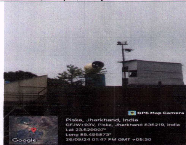
Photo 8: Mist Fogger installed at M/s Bansidhar Construction Private Limited Stone Crusher unit in Piska, Ormanjhi
